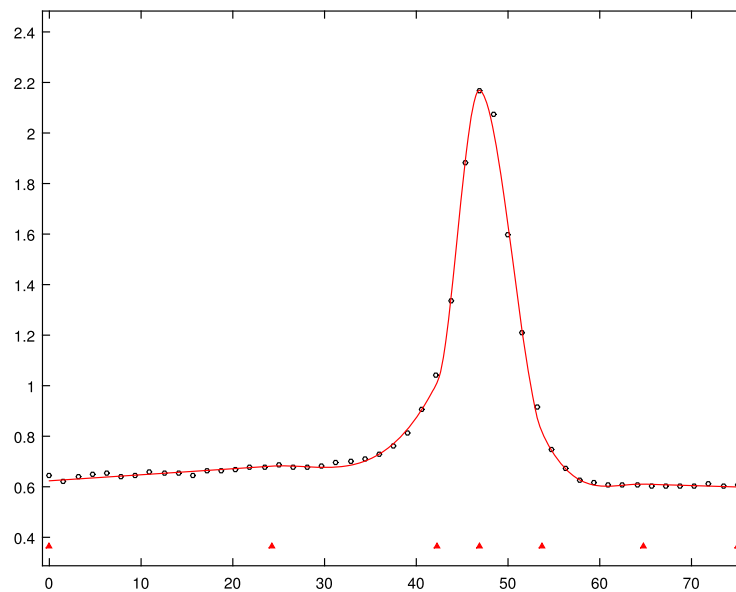
Fig. 6. L^1 spline fit for Titanium heat data. Red triangles indicate the knot locations. Black circles are data points.
