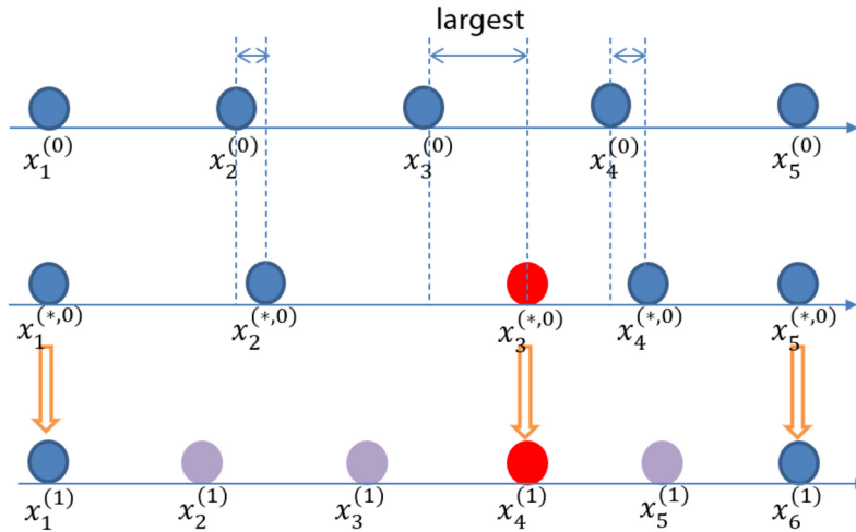
Fig. 1. Illustration of knot number heuristic method: The first iteration, starting with five knots.
