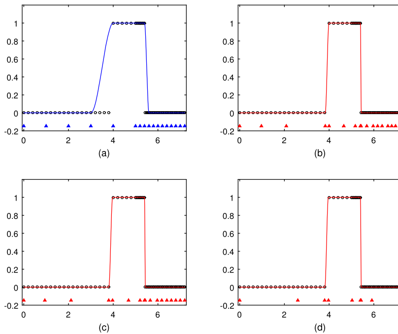
Fig. 2. L^1 spline fits for data set 1: (a) fixed knots (Wang et al., 2014); (b) KLOM with \mathbf{x}^1 ; (c) KLOM with \mathbf{x}^2 ; (d) KNHM. Blue and red triangles indicate the knot locations. Black circles are data points. (For interpretation of the colors in the figure(s), the reader is referred to the web version of this article.)
