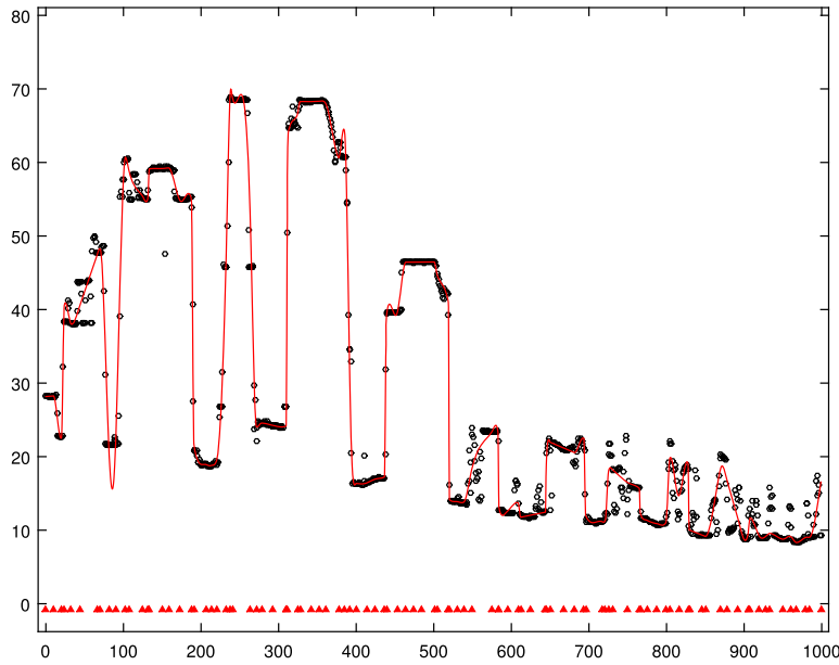
Fig. 7. One of the test data sets with a 100-knot L^1 spline fit. Red triangles indicate the knot locations. Black circles are data points.
