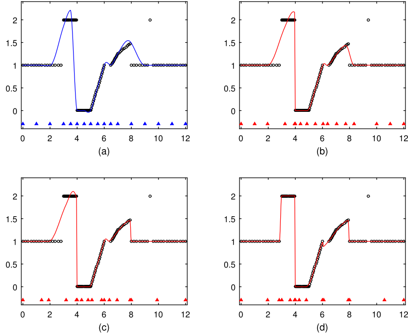
Fig. 3. L^1 spline fits for data set 2: (a) fixed knots (Wang et al., 2014); (b) KLOM with \mathbf{x}^1 ; (c) KLOM with \mathbf{x}^2 ; (d) KNHM. Blue and red triangles indicate the knot locations. Black circles are data points.
