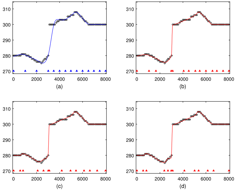
Fig. 4. L^1 spline fits for data set 3: (a) fixed knots (Wang et al., 2014); (b) KLOM with \mathbf{x}^1 ; (c) KLOM with \mathbf{x}^2 ; (d) KNHM. Blue and red triangles indicate the knot locations. Black circles are data points.
